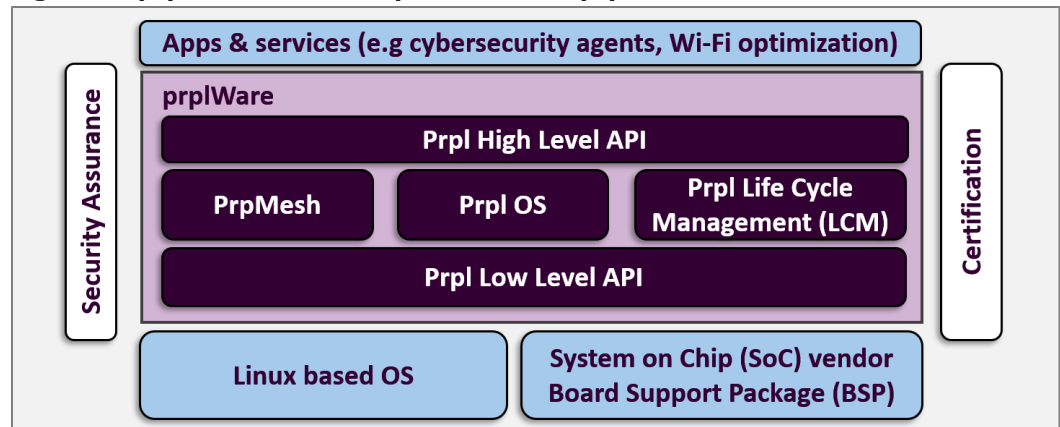
Figure 2: prplWare: The complete suite of prpl software
